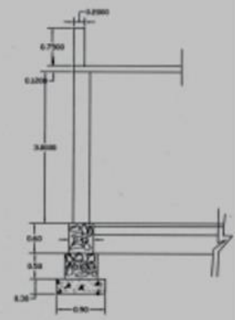
CROSS SECTION AT X-X
